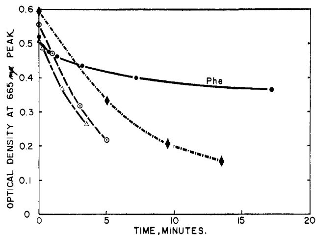
Fig. 6.—Rate of photoreduction of chlorophyllide and pheophorbide in ethanol-pyridine solution; [\text{Asc}] \sim 2 \times 10^{-3} M , I_a \sim 4.5 \times 10^{-6} einstein/l. sec.: ●, [\text{Phe}] = 1.1 \times 10^{-5} M , x_{\text{py}} = 0.105 ; ◆, [\text{Chl}] = 0.86 \times 10^{-5} M , x_{\text{py}} = 0.031 ; △, [\text{Chl}] = 0.76 \times 10^{-5} M , x_{\text{py}} = 0.099 ; ○, [\text{Chl}] = 0.82 \times 10^{-5} M , x_{\text{py}} = 0.103 , like above but in presence of 8.6 \times 10^{-5} M dehydroascorbic acid.
