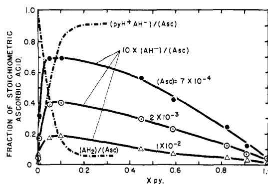
Fig. 3.—Relative amounts of undissociated ascorbic acid [ AH_2 ], free ions [ AH^- ], and ion pairs [ pyH^+AH^- ] in ethanol-pyridine mixtures as fractions of the total concentration [ Asc ]. [ AH_2 ]/[ Asc ] and [ pyH^+AH^- ]/[ Asc ] curves calculated for [ Asc ] = 2 \times 10^{-3} M. Scale for [ AH^- ]/[ Asc ] is enlarged 10 \times .
