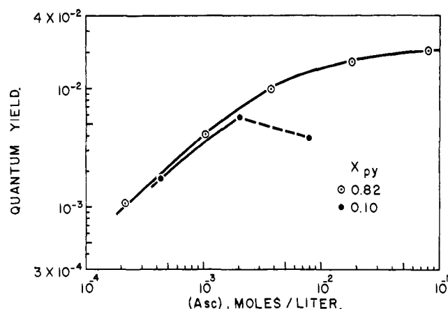
Fig. 5.—Variation of quantum yield for chlorophyllide reduction with ascorbic acid concentration; [\text{Chl}] \sim 8 \times 10^{-6} M , I_a \sim 4 \times 10^{-6} \text{ einstein/l. sec.} Curve through points for x_{py} = 0.82 calculated from eq. 9 with \phi_\infty = 0.021 and K_A = 4.2 \times 10^{-3} M .
